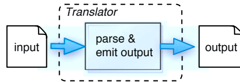
Figure 11.1: Syntax-directed translator
