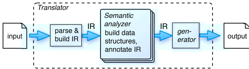
Figure 11.3: Model-driven translator
